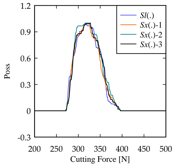
(a) Cutting force for SC15 to SUS304
