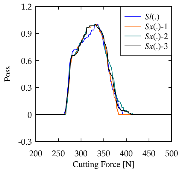
(b) Cutting force for SUS304 to SC15
